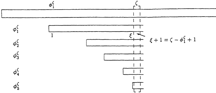
FIG. 4. The algorithm at text position \zeta .
