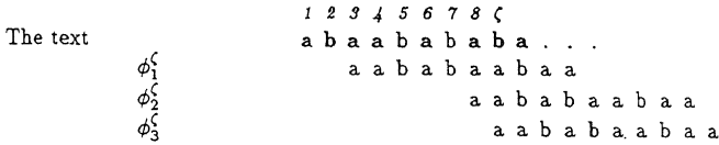
FIG. 1. The state of the algorithm at text position \zeta = 9 . Holes are listed in boldface. Note that there is a hole at text position 9 since symbols at this column in the copies of the pattern aligned starting at text positions in \Phi^{\zeta} = \{3, 8, 9\} are all the same. This means that no comparison is made at this text position and \Phi^{10} will initially inherit all the text positions in \Phi^9 . Later, a comparison must be performed at text position \zeta + 1 = 10 because the column under this position contains different symbols. Since all text positions in \Phi^{10} have credits, the symbol at text position 10 will be compared to "b," the symbol aligned with it in the copy of the pattern that is aligned starting at text position 3, which is the smallest in \Phi^{10} . The comparison fails, \Phi^{10} = \{9, 10\} , and a hole is left at text position 10. If we compared to "a" instead, the comparison would have succeeded and we would have gotten the same set \Phi^{10} , but we would not have a hole at text position 10.
